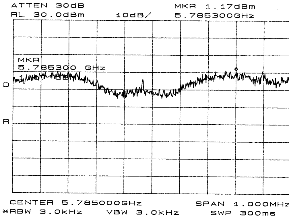
Figure Nineteen Power Spectral Density plot taken in screen room
