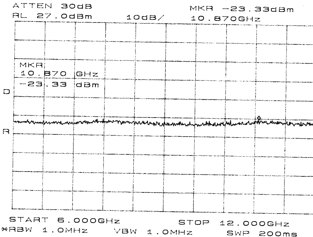
Figure Eleven Antenna Port Conducted Emissions
