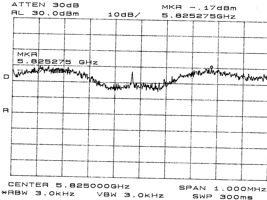
Figure Twenty Power Spectral Density plot taken in screen room
