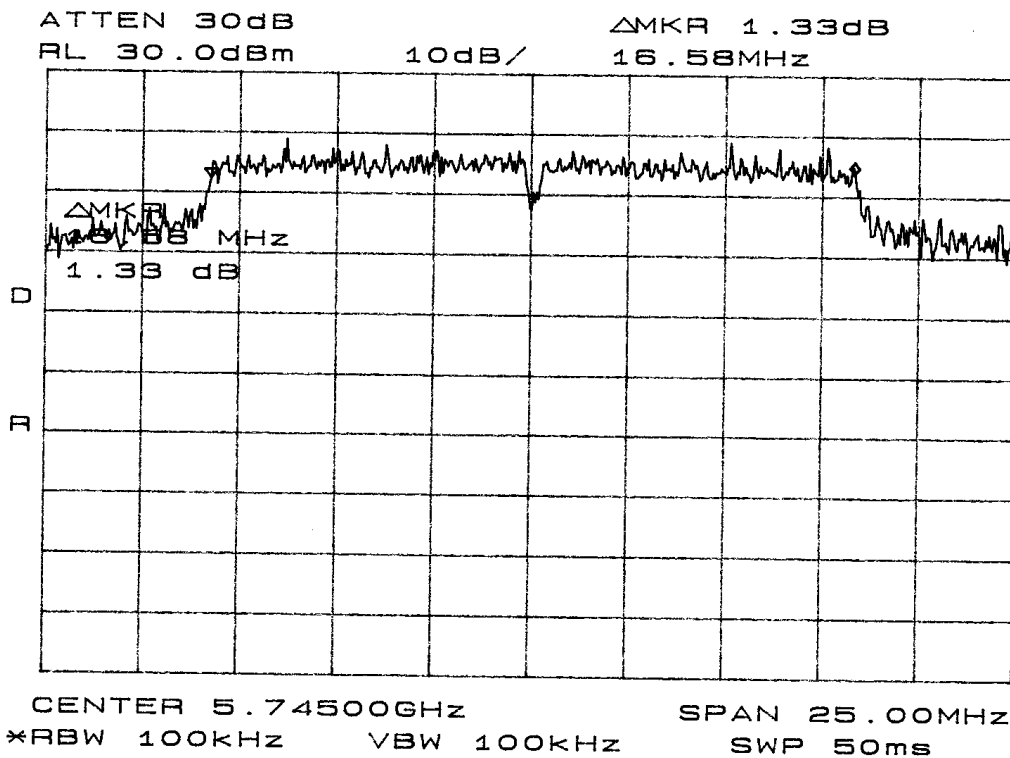
Figure Fifteen 6dB Band width Requirement plot taken in screen room
