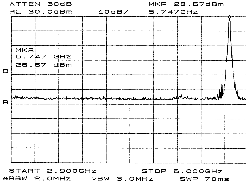
Figure Ten Antenna Port Conducted Emissions
