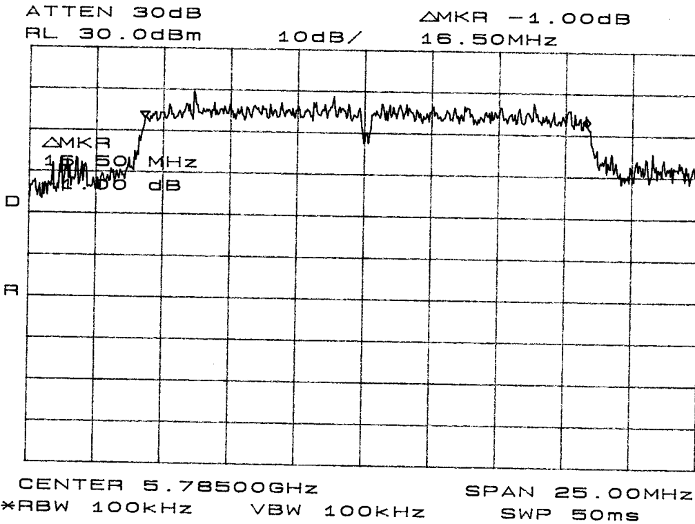
Figure Sixteen 6dB Band width Requirement plot taken in screen room
