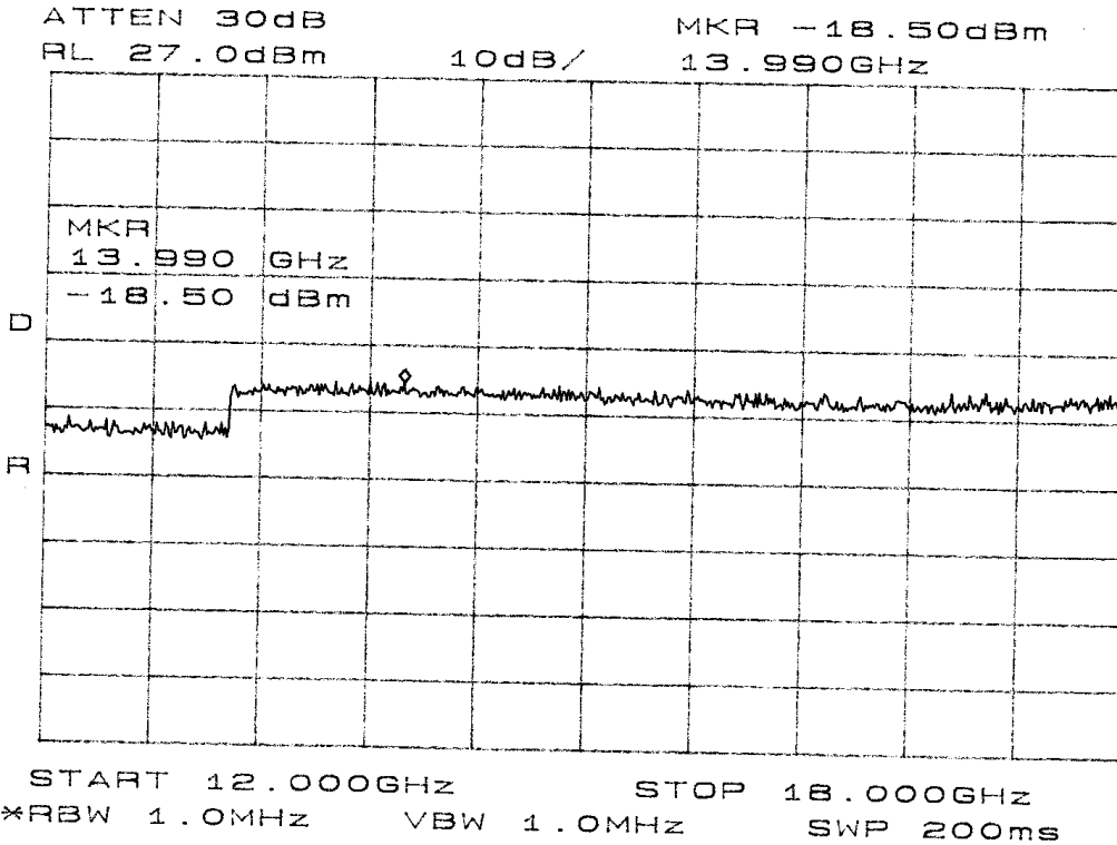
Figure Twelve Antenna Port Conducted Emissions
