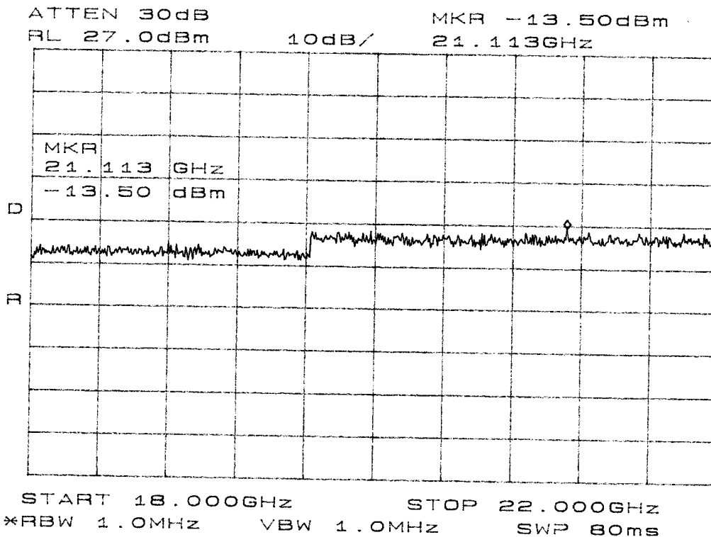
Figure Thirteen Antenna Port Conducted Emissions
