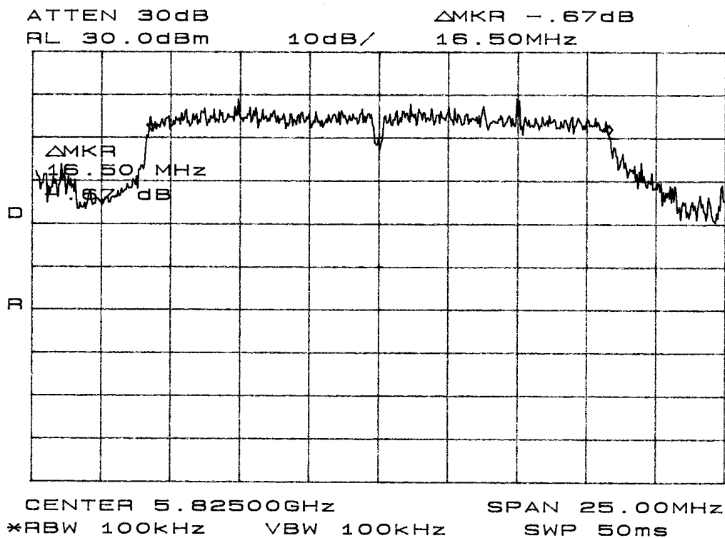
Figure Seventeen 6dB Band width Requirement plot taken in screen room
