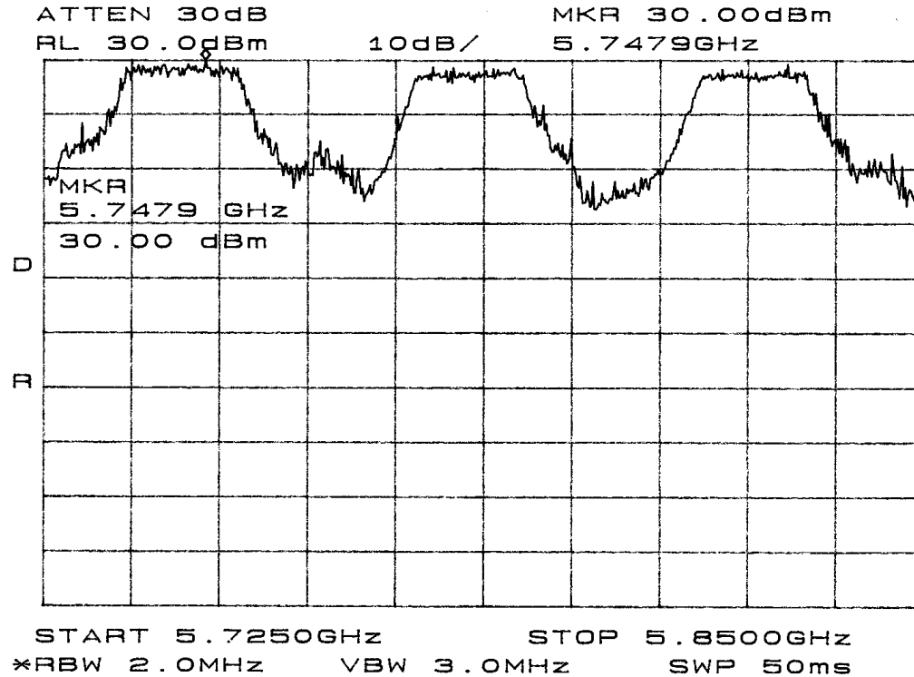
Figure Fourteen Operations at three frequencies in band
